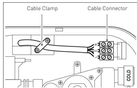
Electrical connections
