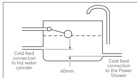
Water tank detail
